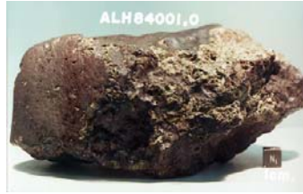
Martian Meteorite
